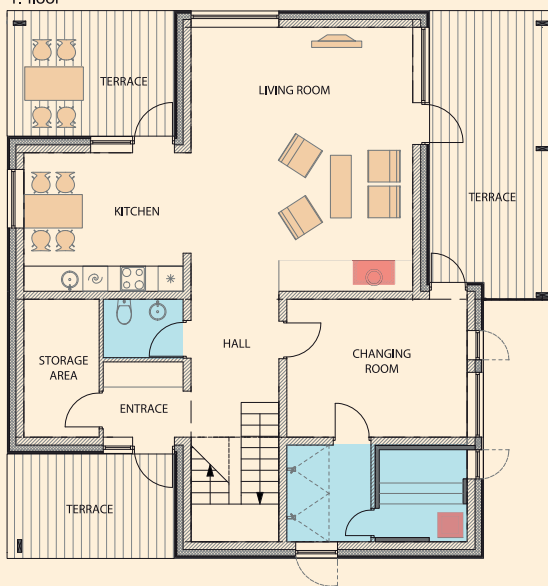
1. floor
